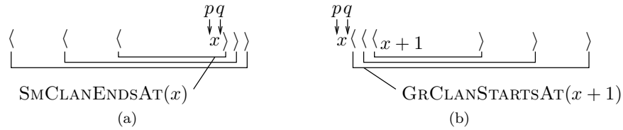
Figure 7: The computation of q in Line 14 (a) and in Line 18 (b).
